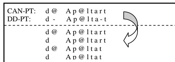
Figure 2: Generation of pronunciation variants through the alignment of two phonetic transcriptions.
